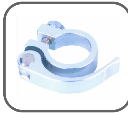
PS-SC07 Specification: \varnothing 25.4/28.6
