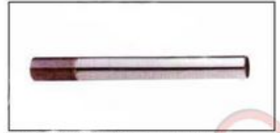
MOD: CP-03 FORK HEAD STEM MATERIAL:STKM11A T:BC1"X24T, 1-1/8"X26T L:160mm-300mm
