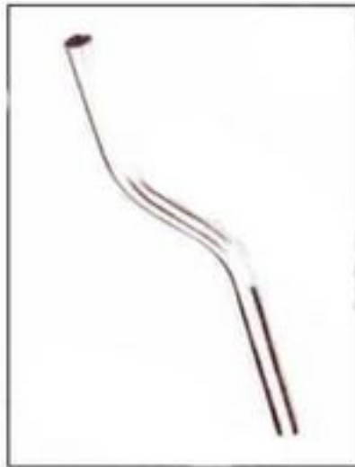
MOD:SP-01 MATERIAL:STEEL DIAMETER:22.2 LENGTH:370mm FINISH:CP
