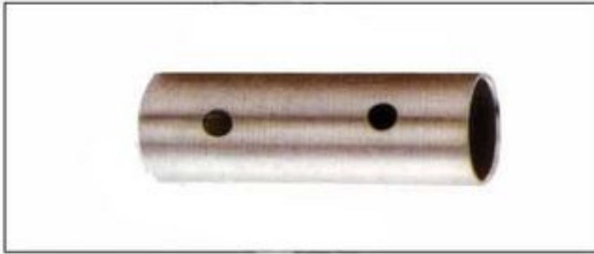
MOD: LS-01 HEAD LUG MATERIAL:STKM11A OD:38mm ID:34mm OD:34mm ID:30mm LENGTH:85-200mm
