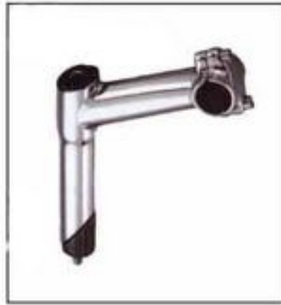
MOD:HS-011 MATERIAL:STEEL EXT:100mm RISE:10DEG QUILL:150mm-180mm FINISH:CP
