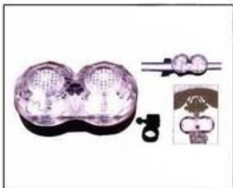
MOD: DL-600T: Tail light red color. DL-600F: Front light white color. 4 Flashing functions 2 super bright LED. Battery: 2XAAA
