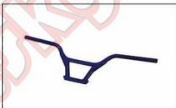
MOD:HL-877 WIDTH:690mm RAISE:190mm
