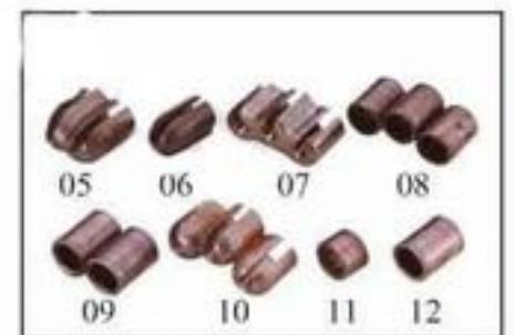
MOD:CB-05,06,07,08,09,10,11,12 SLOTTED CABLE STOP. STEEL BRONZE WELD HOLE DIA:Φ6.3
