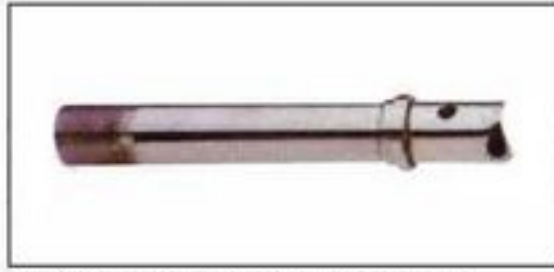
MOD: CP-02 FORK HEAD STEM MATERIAL:STKM11A T:BC1"X24T, 1-1/8"X26T L:160mm-300mm
