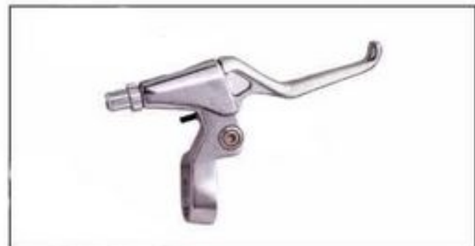
MOD:BL-22 MATERIAL:LIGHT-ALLOY SUITABLE FOR V-BRAKE 3 FINGER, RETURN SPRING
