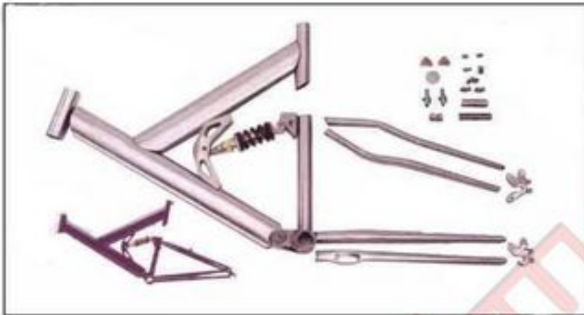
MOD: NF-20 MATERIAL: STEEL FINISH: WITHOUT PAINTED UN-WELDED FRAME
